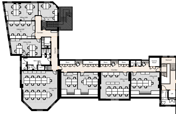
1 Second Floor Scale: 1:200
